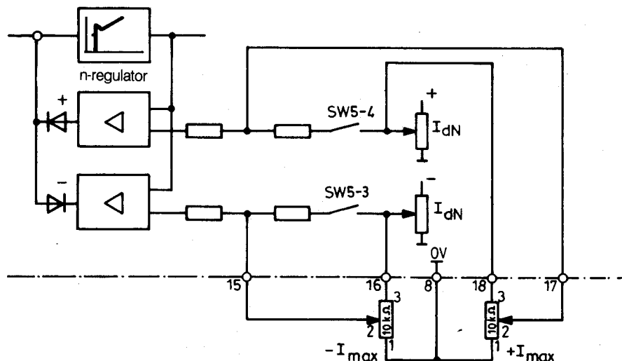
Fig. 5.5.2.1 External current limitation
