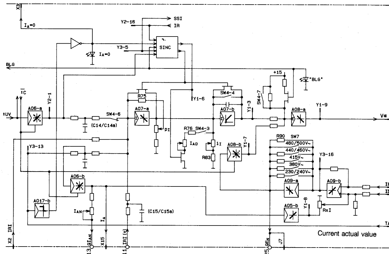
Fig. 5.7.1 Current regulator
